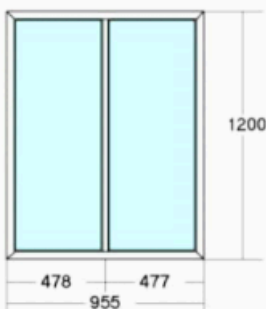
Half Opening window 1200H x 955W
