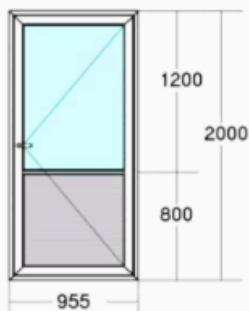
Half Glazed Door 2000H x 955W
