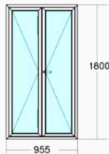
French Window 1800H x 955W
