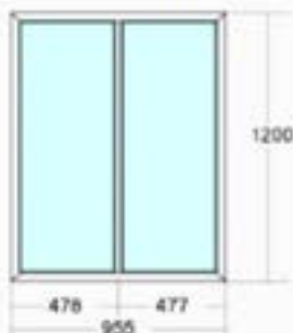
Half Opening window 1200H x 955W
